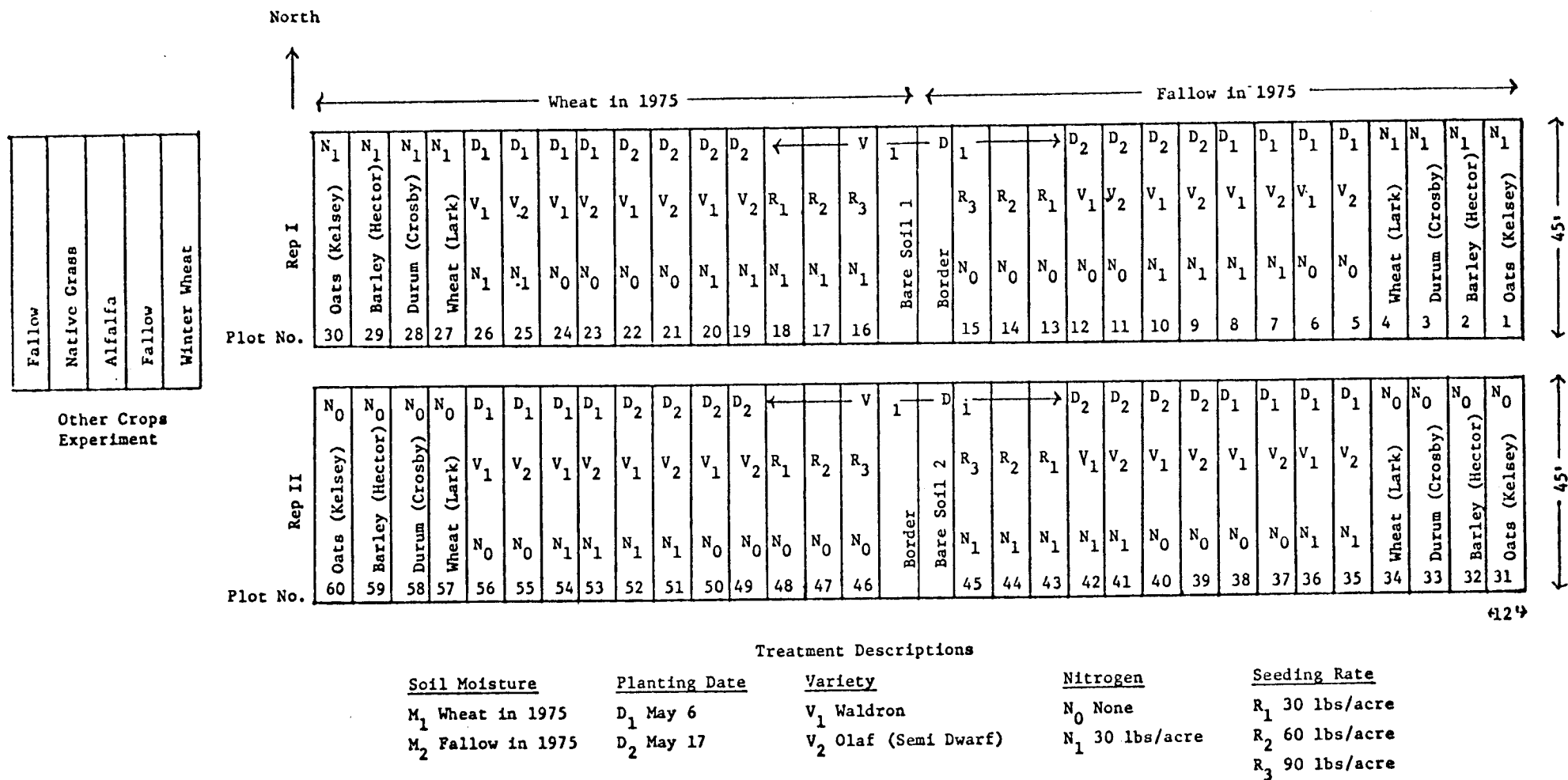
Figure 46.1 Design for 1976 Seeding Rate Experiment
